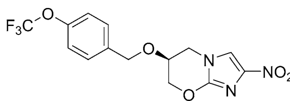
Fig. 3. Chemical structure of pretomanid (PTM; 3)
