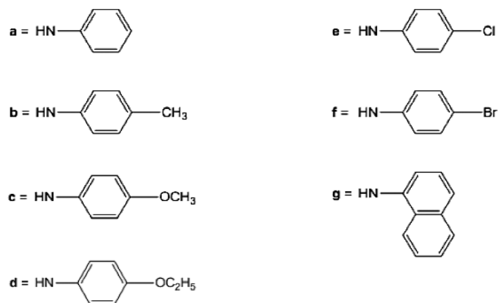
Fig. 3. Acetylpyrazine thiosemicarbazones modified in the thiosemicarbazide moiety
