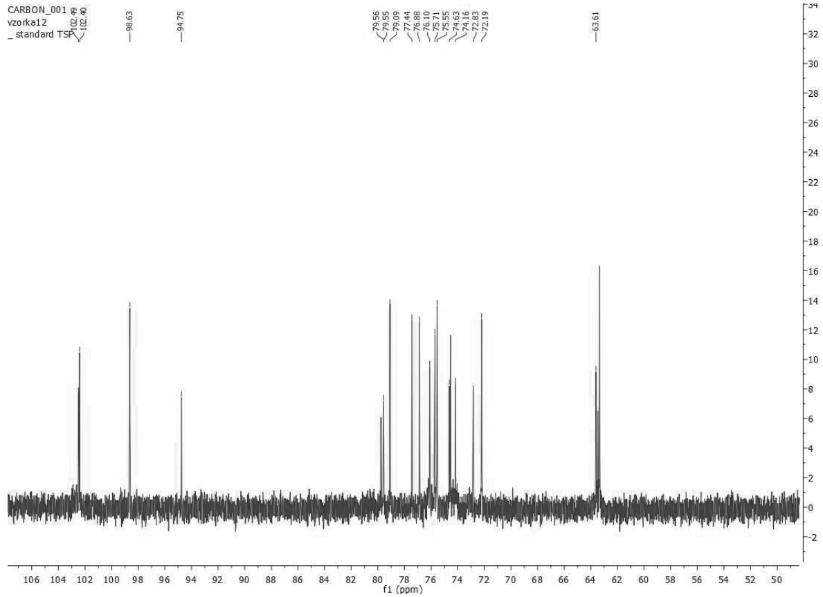
Fig. 5. 13 C NMR spectrum of the CBHP polysaccharide
