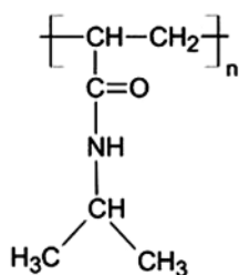
Fig. 3. The chemical structure of pNIPAAm
