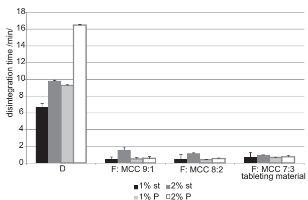
Fig. 4. Disintegration time of tablets at the compression force of 14 kN D – Disintequik™ MCC, F – Flowlac® 100, MCC – Microcel® MC-102, st – magnesium stearate, P – poloxamer 407
