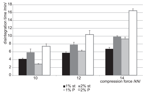
Fig. 3. Disintegration time of tablets in function of compression force – Disintequik™ MCC with lubricants st – magnesium stearate, P – poloxamer 407
