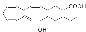
15-(S)-HETE
