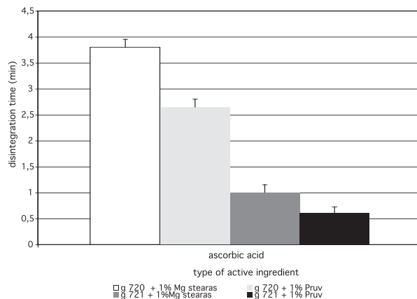
Fig. 6. Disintegration time of tablets at the compression force of 10 kN: galen IQ 720 and 721 with ascorbic acid g 720 – galenIQ 720, g 721 – galenIQ 721, Mg stearas – magnesii stearas
