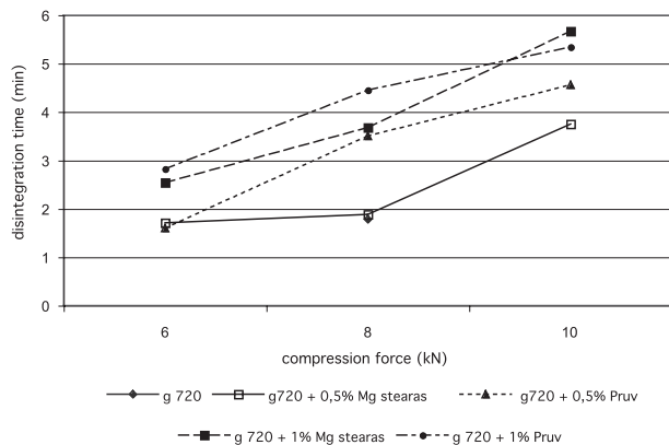
Fig. 3. Disintegration time in function of compression force: galen IQ 720 g 720 – galenIQ 720, Mg stearas – magnesii stearas
