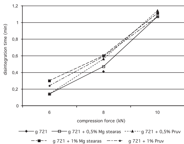
Fig. 4. Disintegration time in function of compression force: galen IQ 721 g 721 – galenIQ 721, Mg stearas – magnesii stearas
