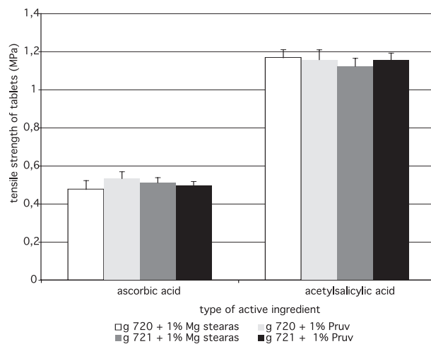
Fig. 5. Tensile strength of tablets at the compression force of 10kN: galen IQ 720 and 721 with active ingredients g 720 – galen IQ 720, g 721 – galenIQ 721, Mg stearas – magnesii stearas
