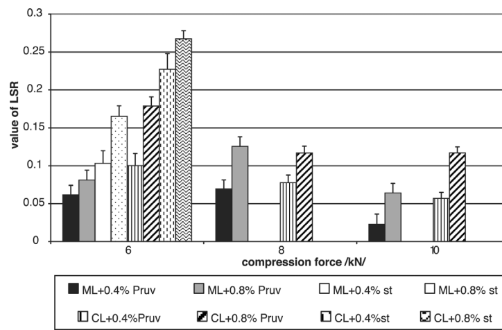
Fig. 5. Values of LSR for MicroceLac®100 and Cellactose®80
